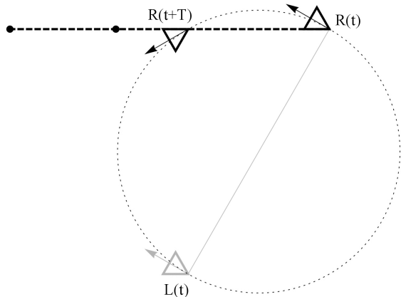
Figure 1. For a stereo rig with parallel cameras L and R, we consider two scene points (indicated by small black circles) that lie in the plane that contains the stereo camera motion and that enter and then exit the field of view of the right camera at times t and t+T respectively. Note that the points are colinear with these two camera positions.
