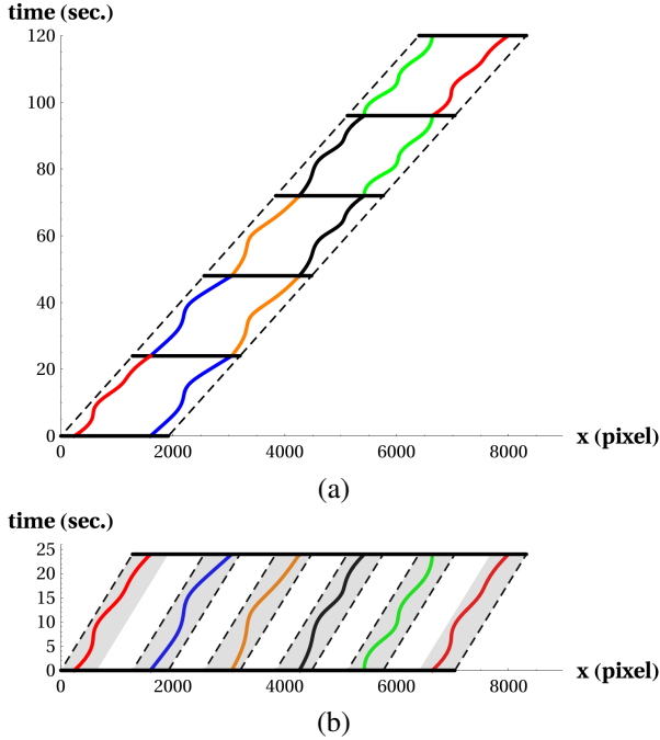
Figure 2. For a frame sequence captured by a camera performing a full turnaround in N = 5T seconds at constant speed, the cut finds a low cost seam between the right border of a frame and the left border of frame T seconds later. (a) The continuous cut shown twice in the full original space-time volume divided in five non-overlapping blocks. (b) The same continuous cut shown with blocks aligned to start at the same time. The overlap regions are indicated in gray.
