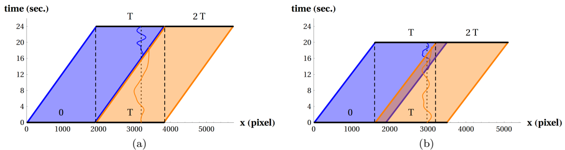
Fig. 2. (a) The motion of a visible scene point is continuous at the temporal boundary (horizontal edge), but there will be a motion discontinuity at the spatial boundary (seam), namely the diagonal edge in this figure. (b) For an object moving in time (a leaf, for instance), motion is blended over the overlap between the two blocks.
