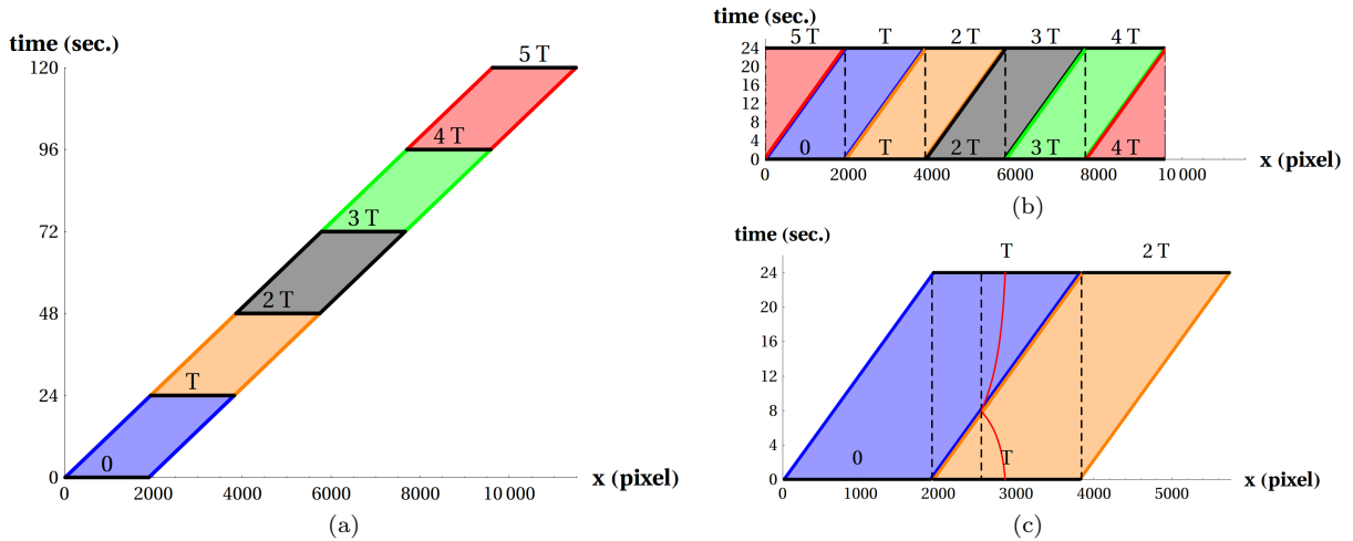
Fig. 1. For a frame sequence captured by a camera performing a full turnaround in N = 5T seconds at constant speed: (a) the full original space-time volume divided in five non-overlapping blocks. (b) The blocks are aligned to start at the same time. (c) Motion paths of two static objects, one far away (central dashed vertical line) and one close-by (red curve). The curve in the latter is caused by motion parallax, that is, the cameras rotating off-axis. Despite using full frames, the motion paths are continuous and loopable.
