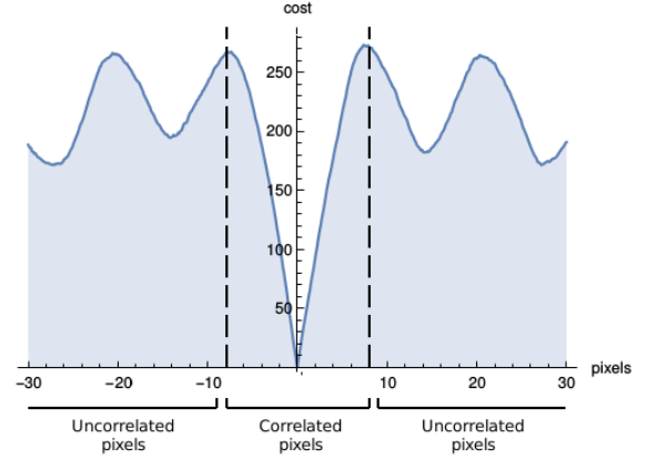
Figure 6: Cost function curve which shows that within a specific neighborhood, \pm 10 pixels in this case, in the unstructured light pattern, the cost is monotonous and easy to minimize.
