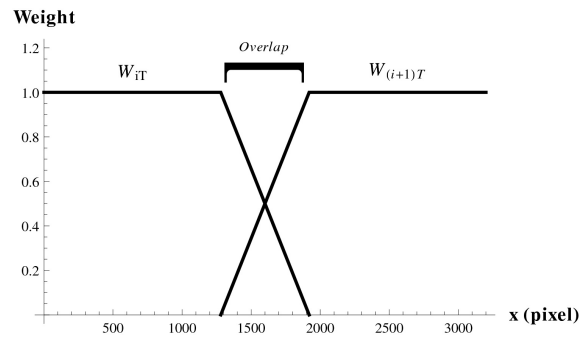
Figure 2.9. Blending function for overlapping frames. Weighting functions W_{iT}(x) and W_{(i+1)T}(x) are given in Sec. 2.3.5.
