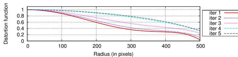
Fig. 8. The distortion function of the fisheye lens, at different iterations of the calibration algorithm for an initial center very far from the true position (200,400). The final estimate of (512,523) was found in only 5 iterations (image of size 1000 \times 1000 pixels). Subsequent steps were only minor improvements.
